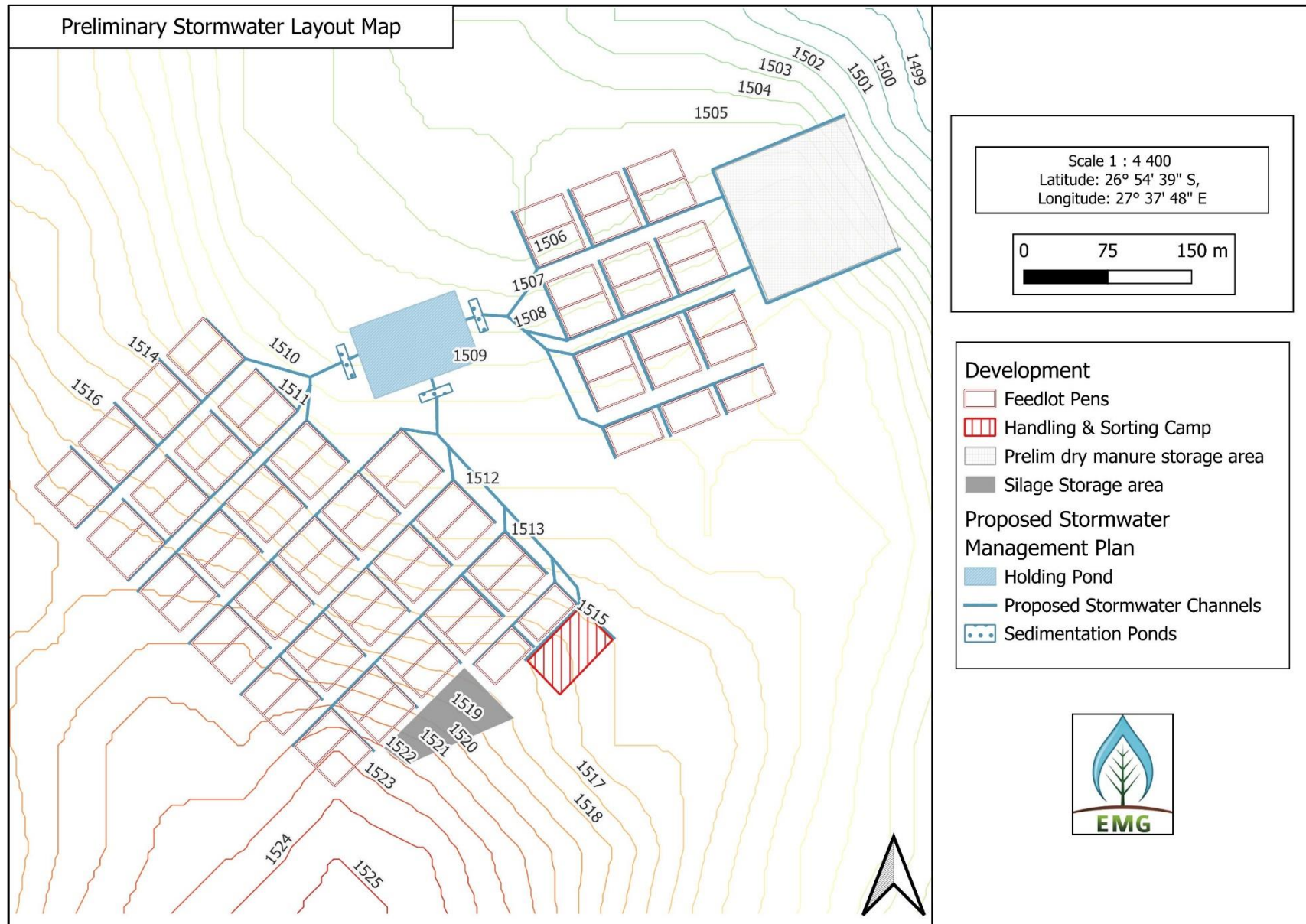
Figure 1 Proposed Stormwater Management Plan for the feedlot development. The holding pond, stormwater channels and sedimentation pond are indicated on the map, as well as the elevation of the area.
