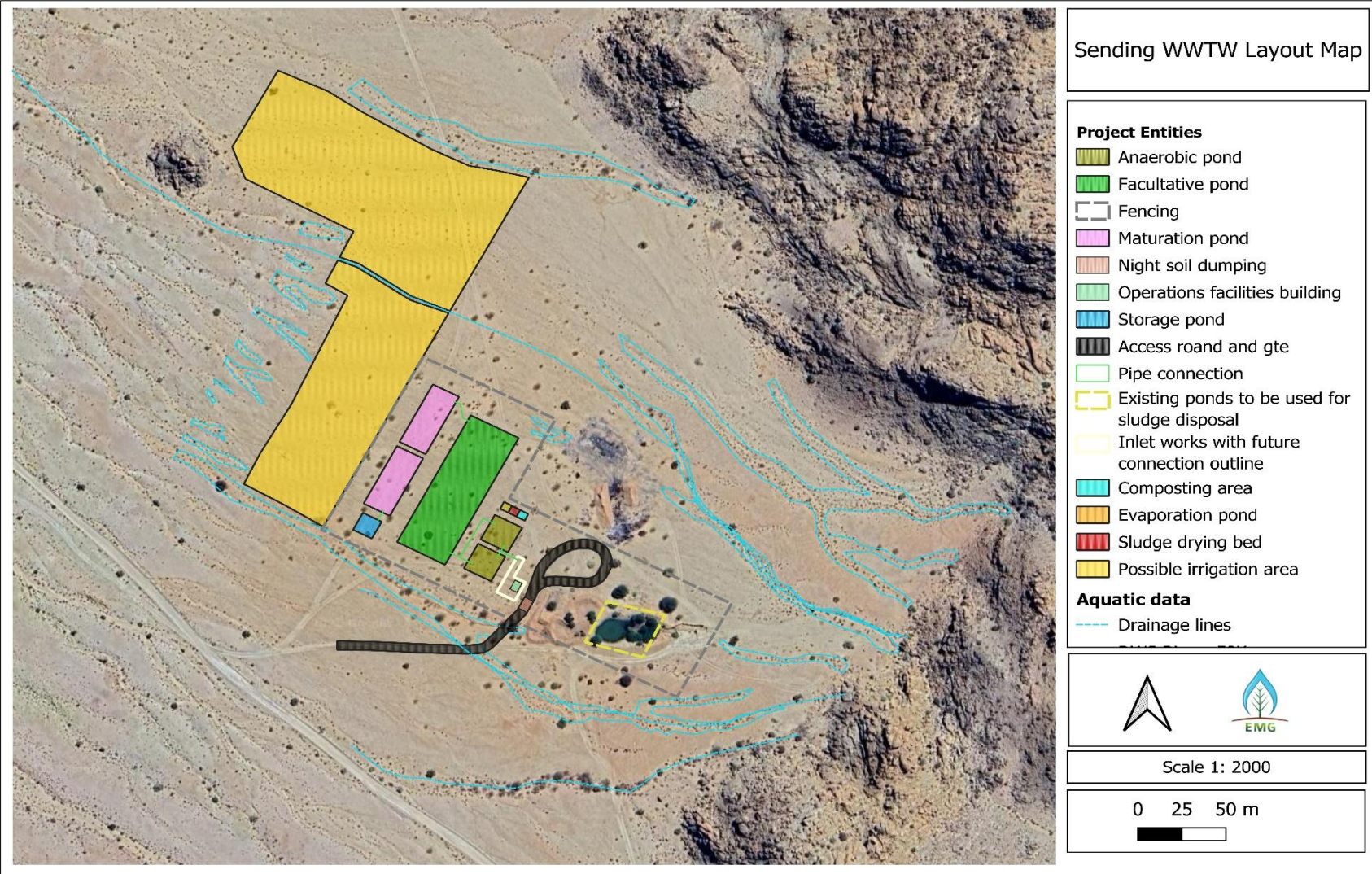
Figure 1 Proposed site layout for the Sending WWTW upgrade, depicting the spatial arrangement of the anaerobic, facultative, and maturation ponds and related works
