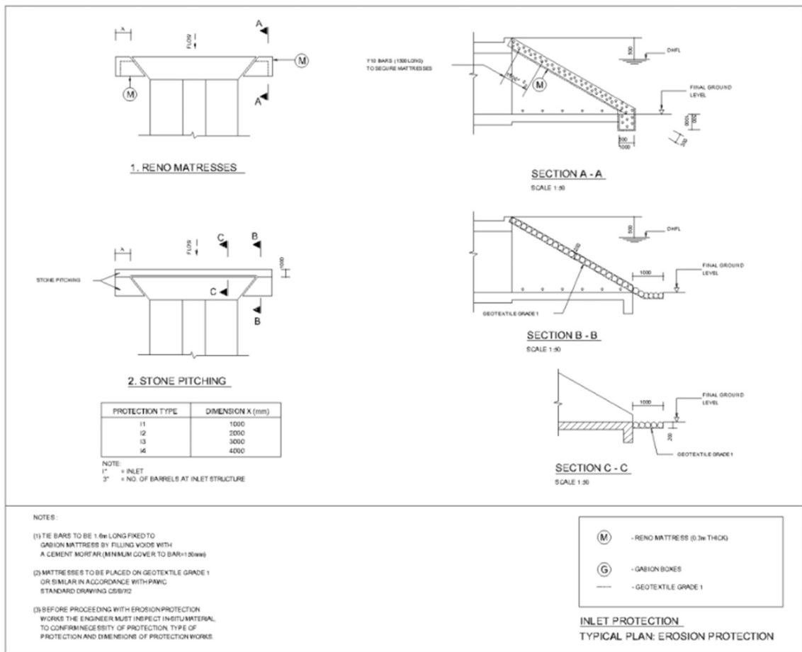
Figure 5: Typical inlet erosion protection.
