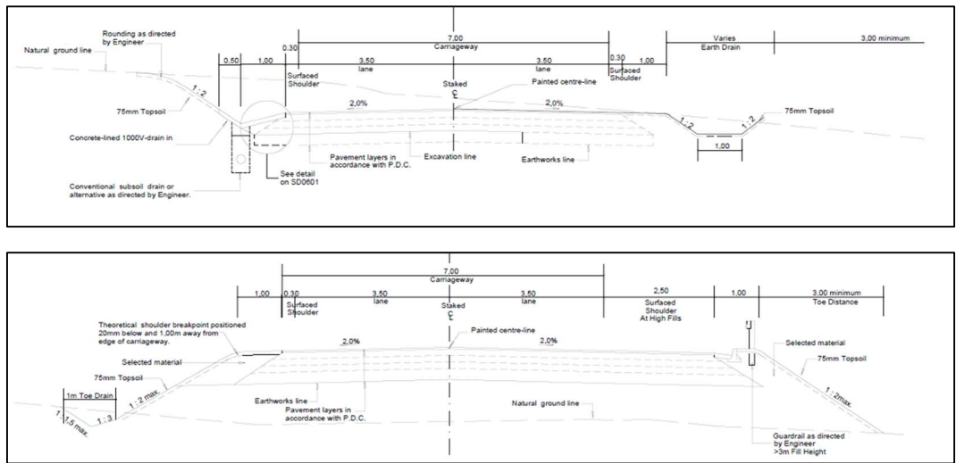
Figure 1: Typical Cross-Section Design for the DR3342 Road Upgrade.
