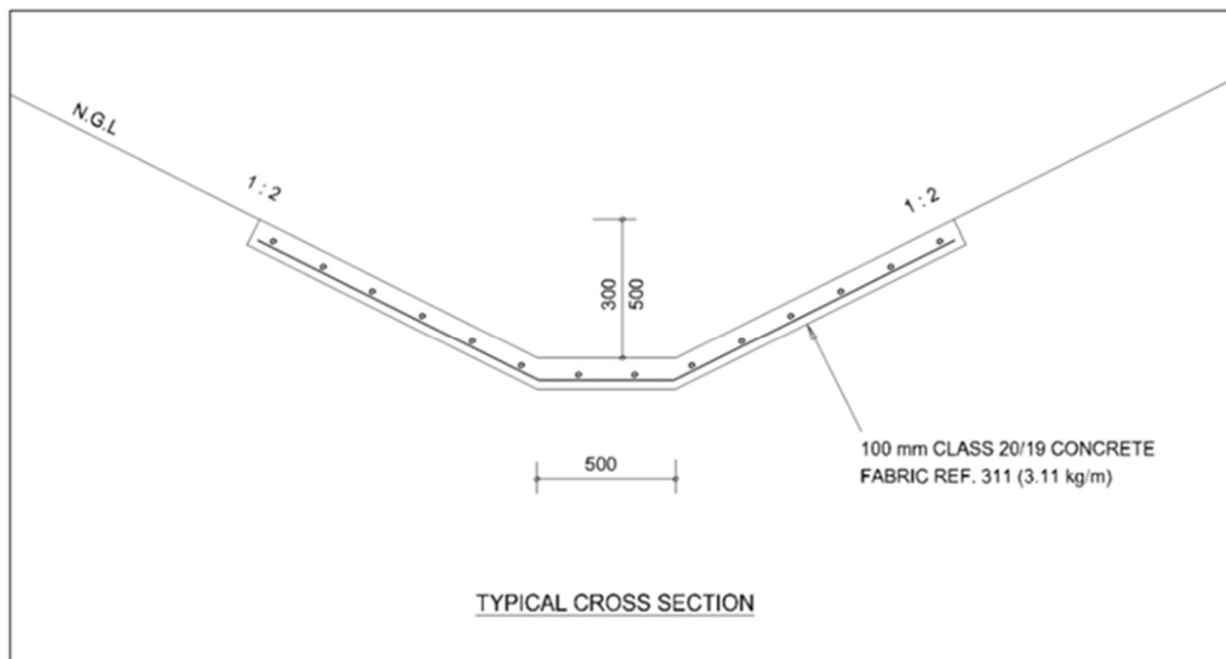
Figure 3: Typical Concrete Lined Side drain.
