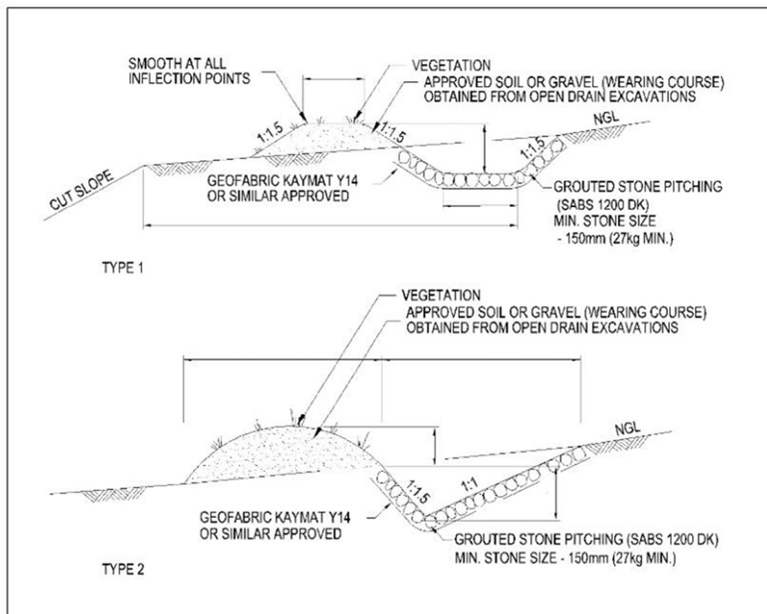
Figure 4: Typical berm and cutoff drain detail.
