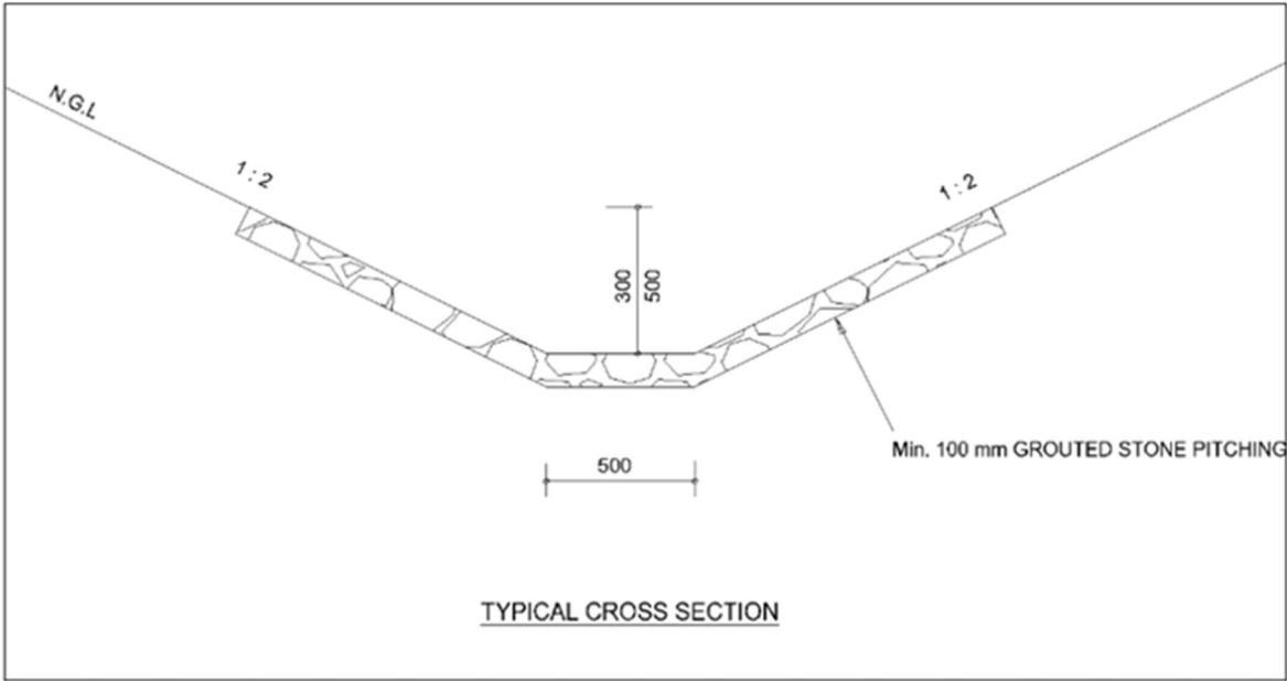
Figure 2: Typical stone pitched side drain.
